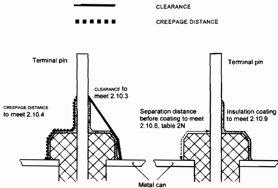
Figure A-10 – Coating around terminals
