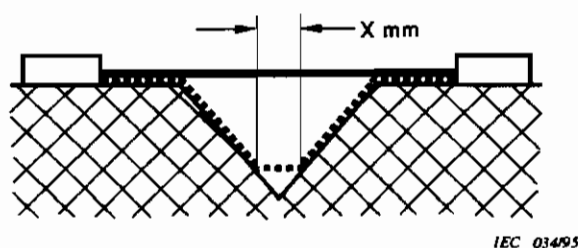
Figure A-2 – Wide groove
